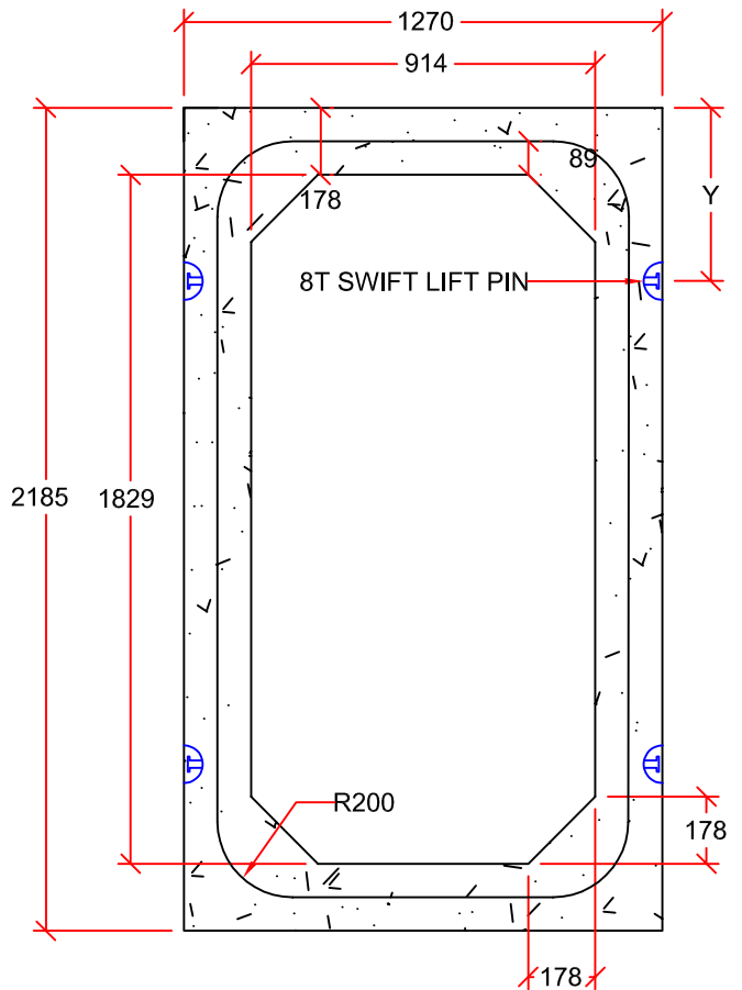
CROSS-SECTION
