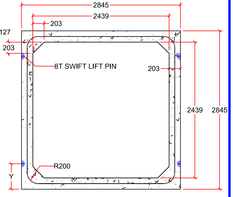
CROSS-SECTION
