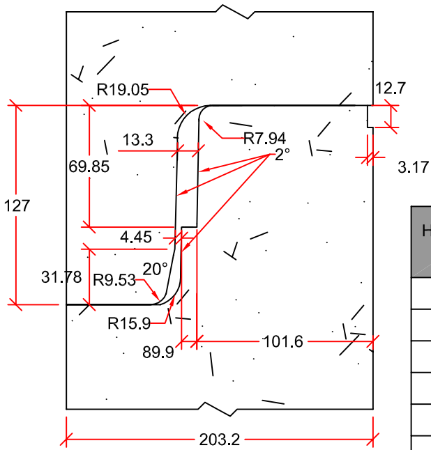
JOINT DETAIL
