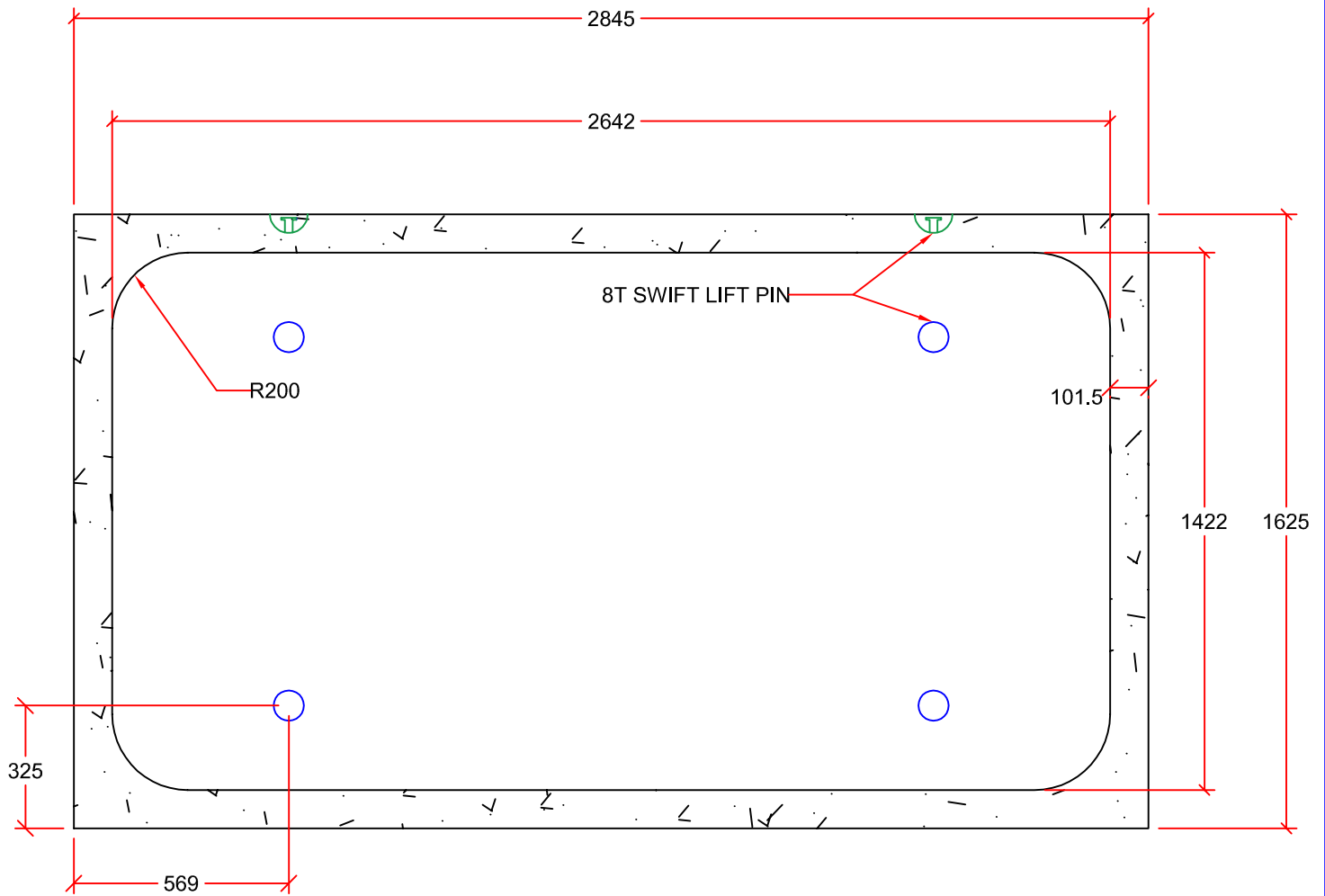
PLAN VIEW
