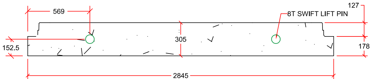
PROFILE VIEW
