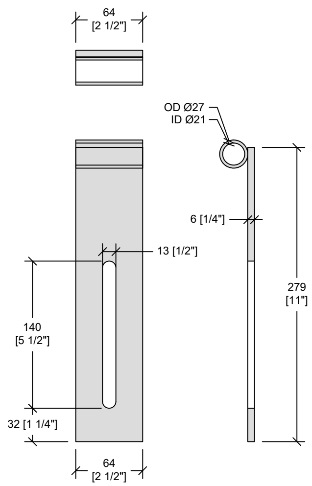
MOUNTING PLATE DETAIL
