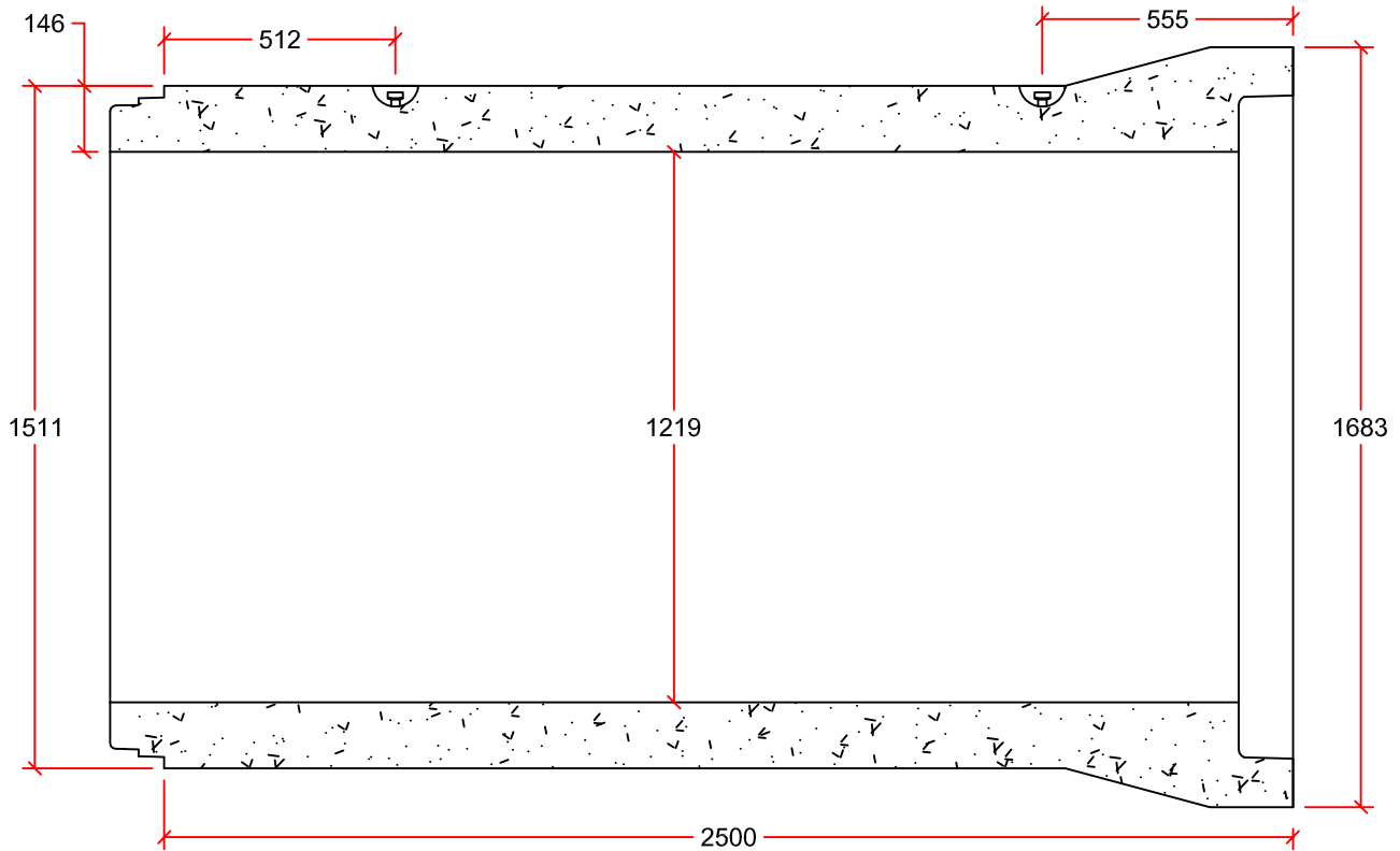
PIPE DETAIL
