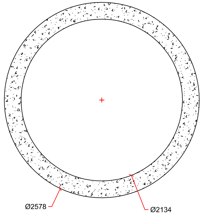
SECTION DETAIL
