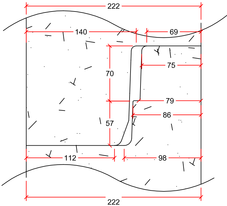
JOINT DETAIL
