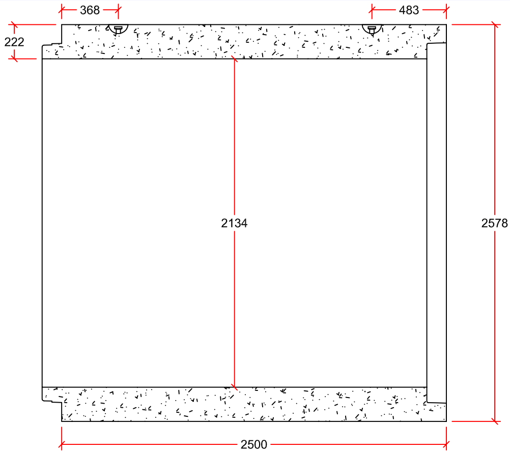
PIPE DETAIL
