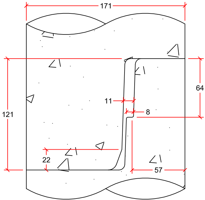
JOINT DETAIL
