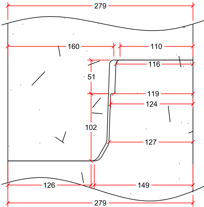
JOINT DETAIL
