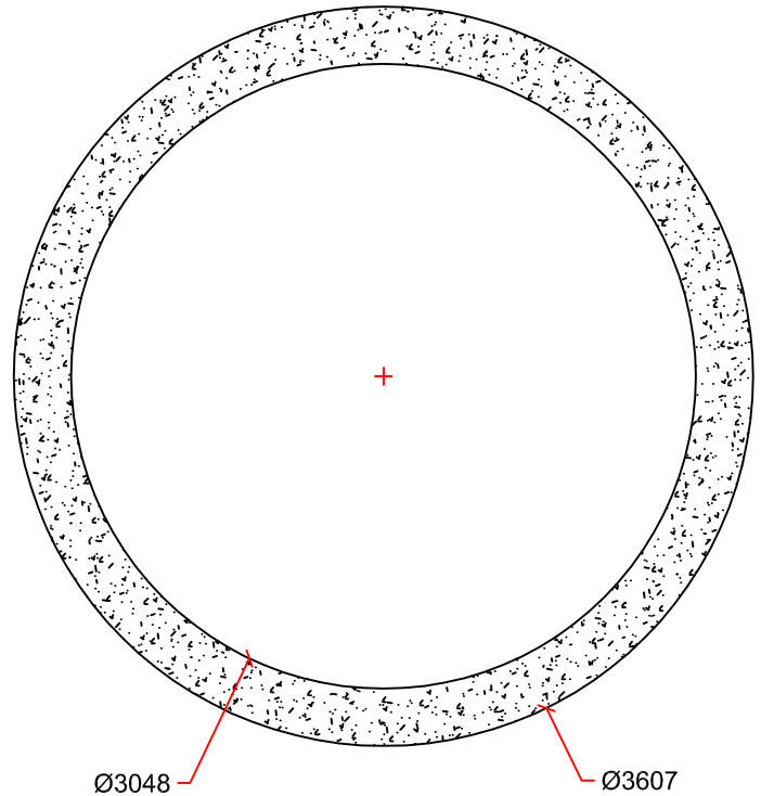
SECTION DETAIL
