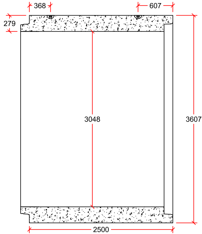
PIPE DETAIL
