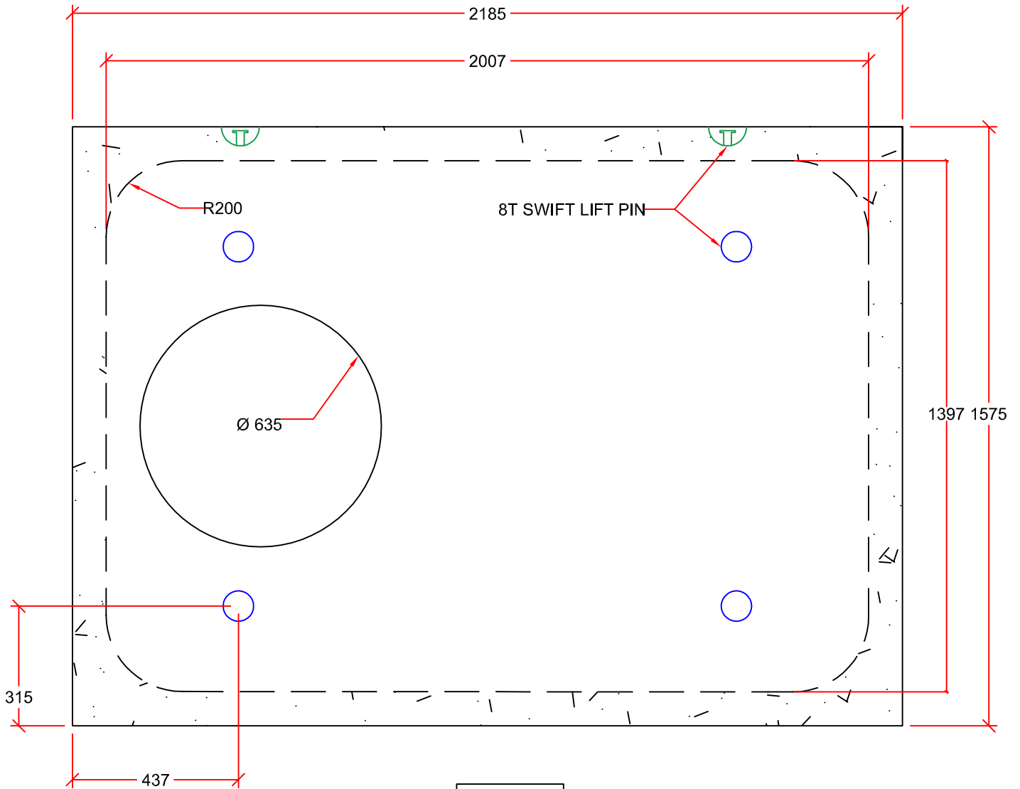
PLAN VIEW
