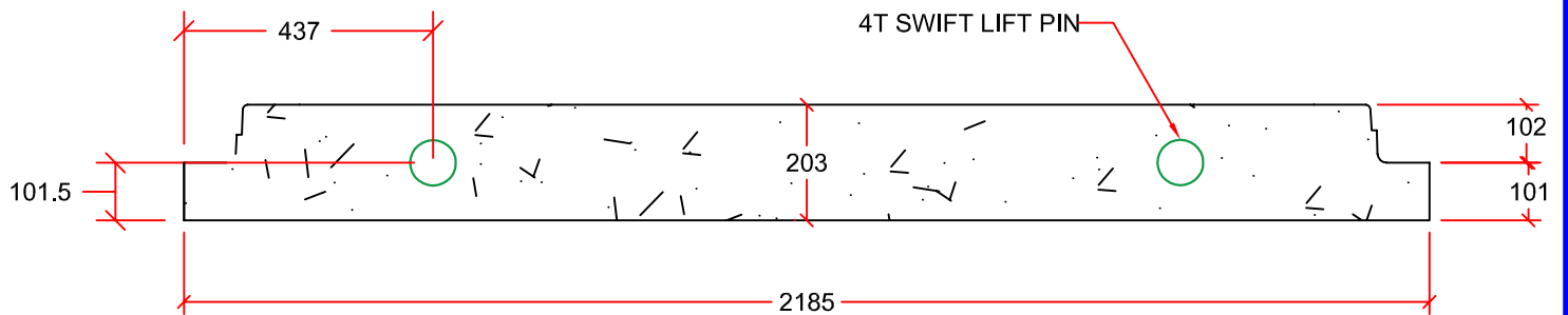
PROFILE VIEW
