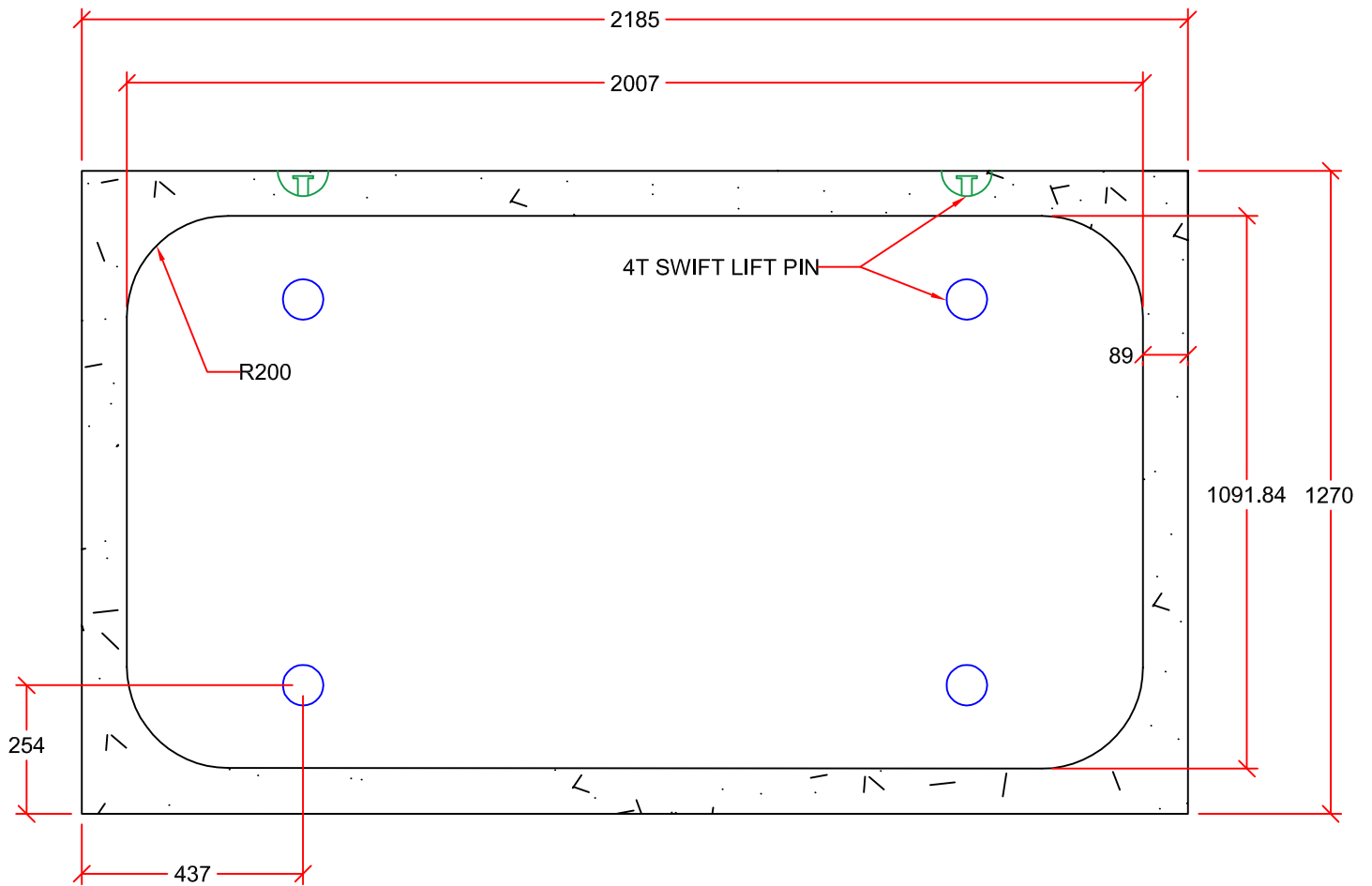
PLAN VIEW
