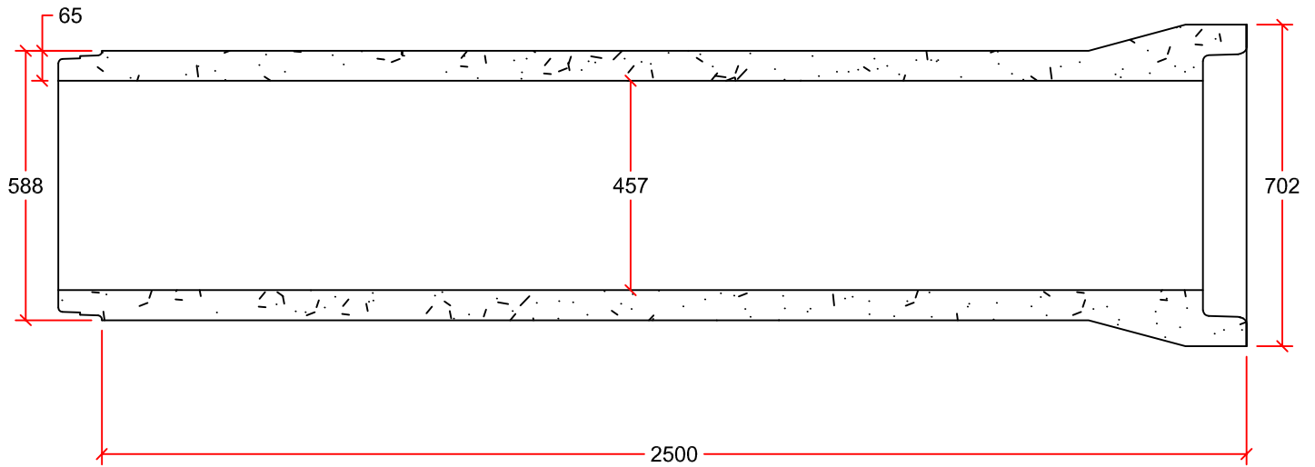
PIPE DETAIL
