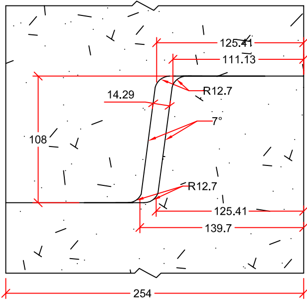
JOINT DETAIL
