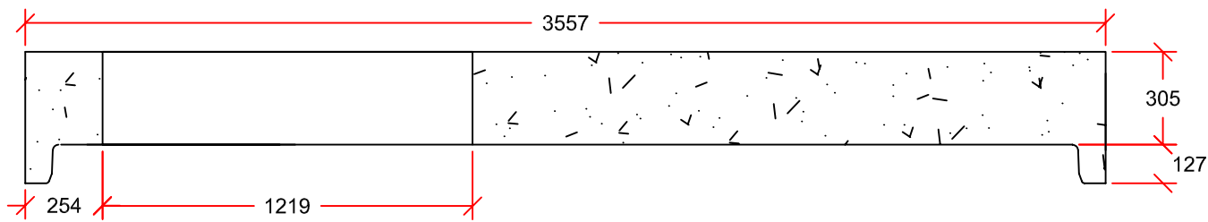
PROFILE VIEW
