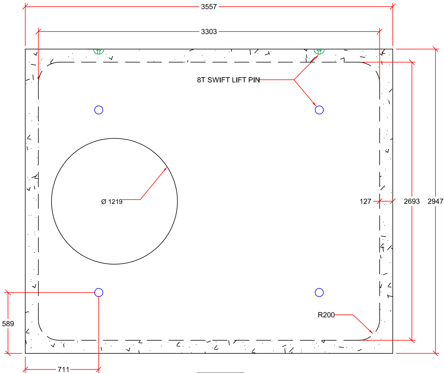
PLAN VIEW
