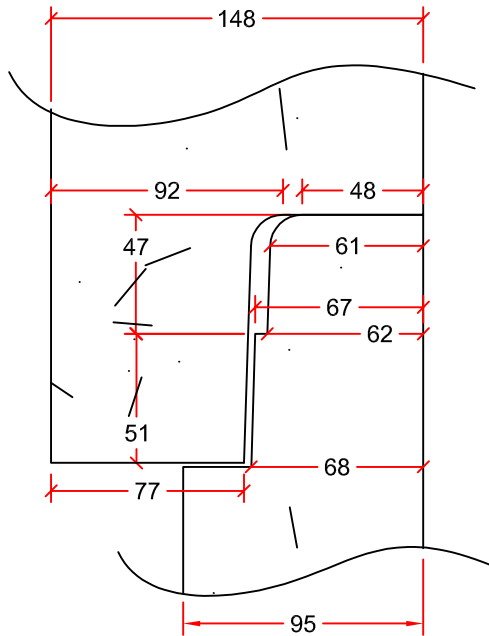
JOINT DETAIL
