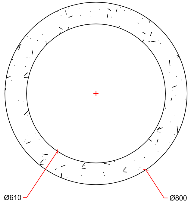
SECTION DETAIL
