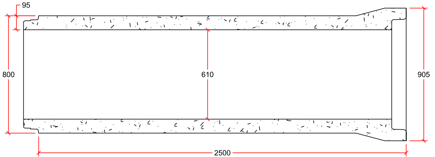
PIPE DETAIL
