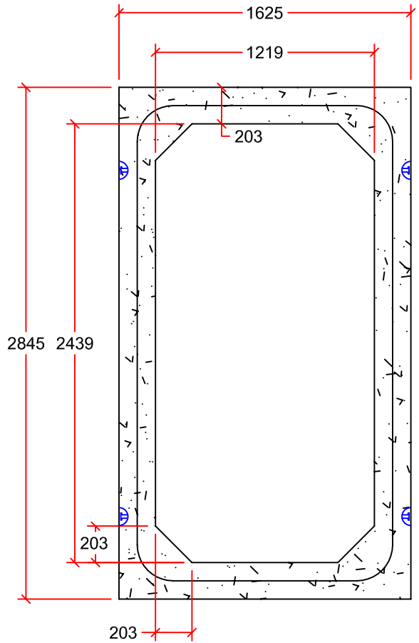
CROSS-SECTION
