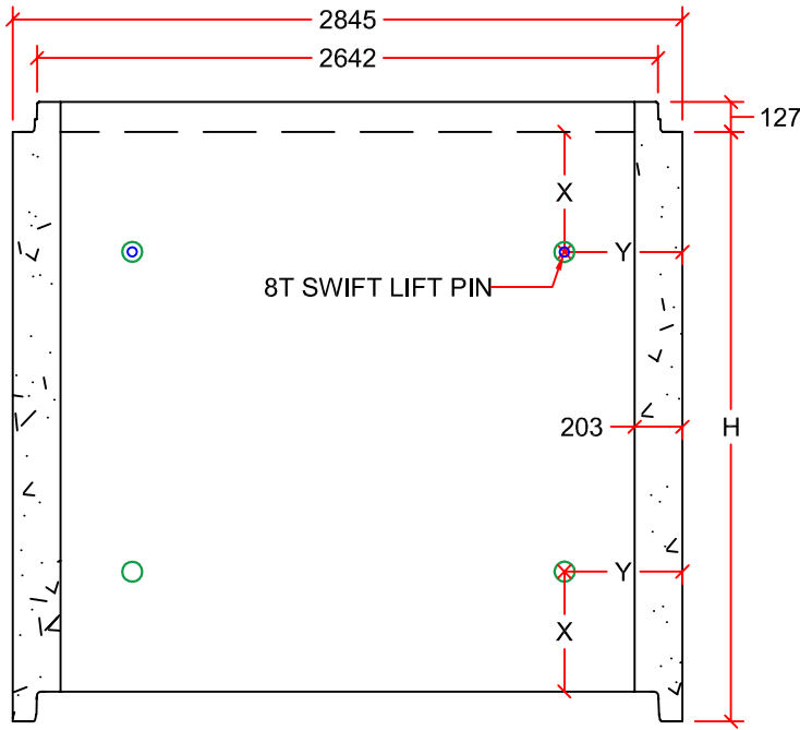
PROFILE VIEW
