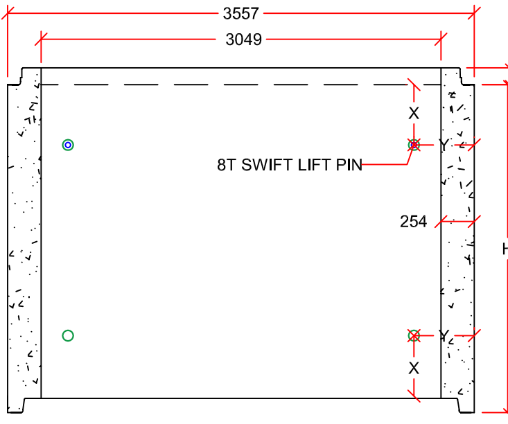
PROFILE VIEW
