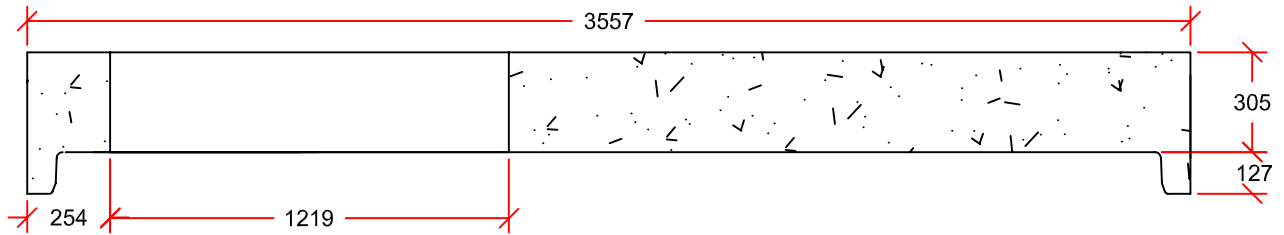
PROFILE VIEW
