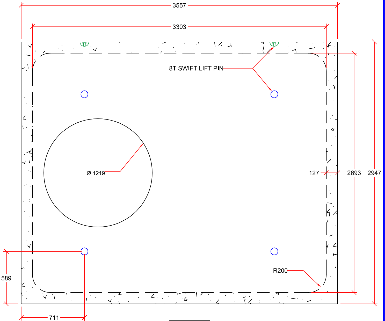
PLAN VIEW
