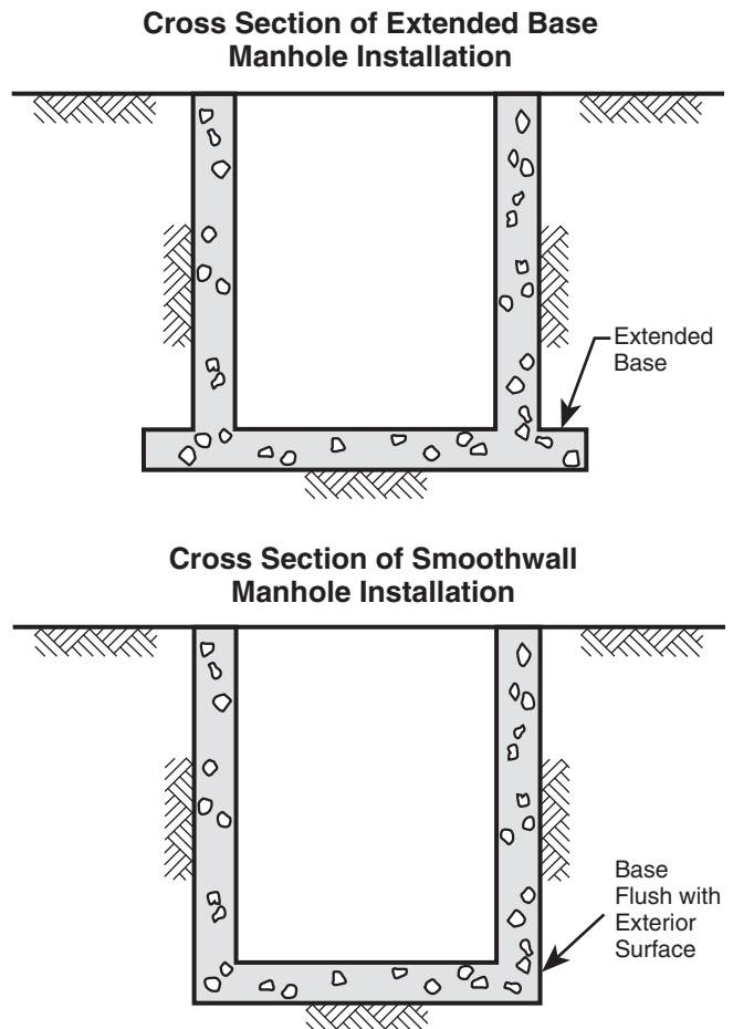
Figure 1 Manhole Installations
