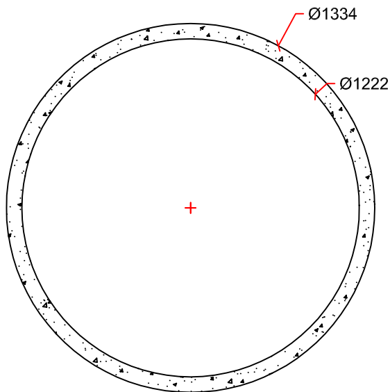
SECTION DETAIL
