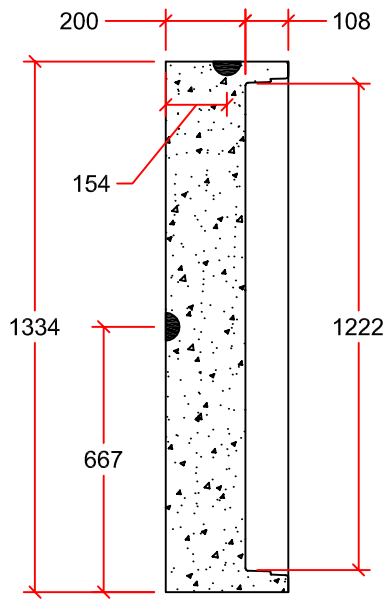
PROFILE VIEW
