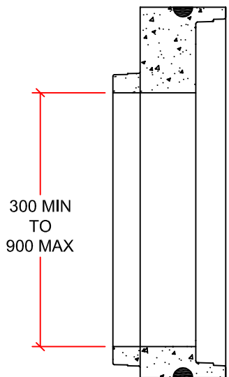
DECREASER
