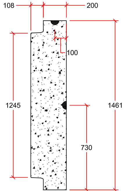
PROFILE VIEW
