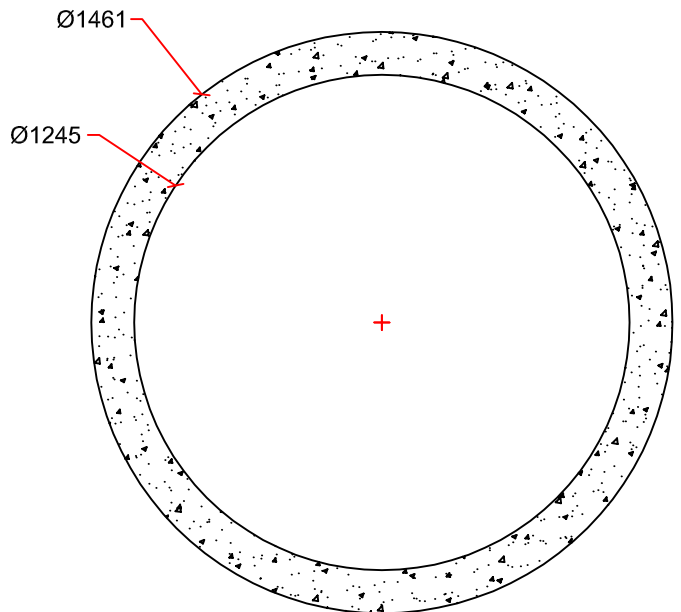
SECTION DETAIL
