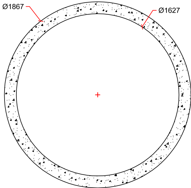
SECTION DETAIL
