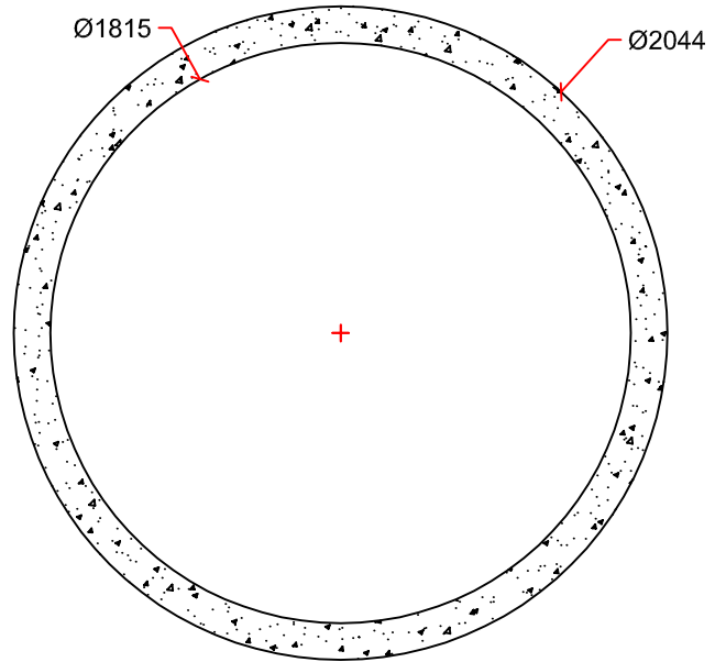
SECTION DETAIL
