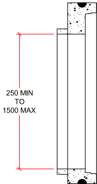
DECREASER
