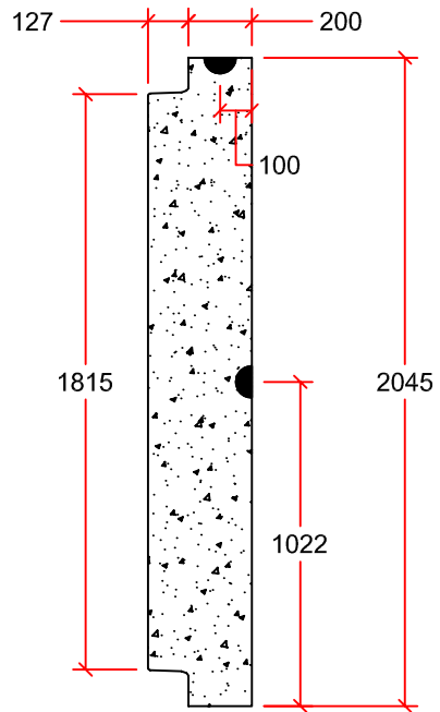
PROFILE VIEW
