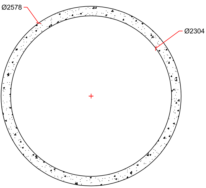
SECTION DETAIL
