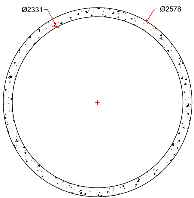
SECTION DETAIL
