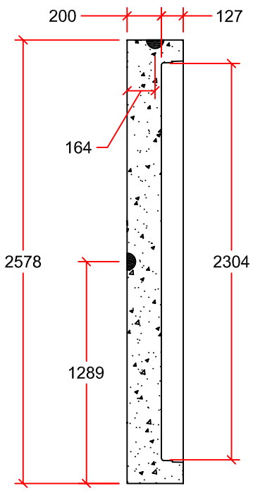
PROFILE VIEW
