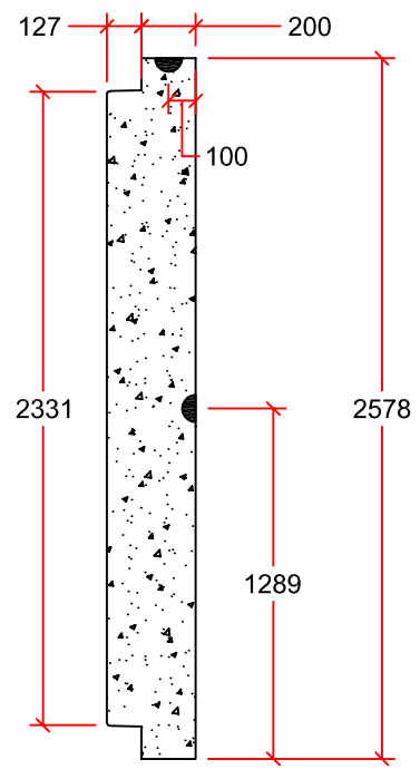
PROFILE VIEW
