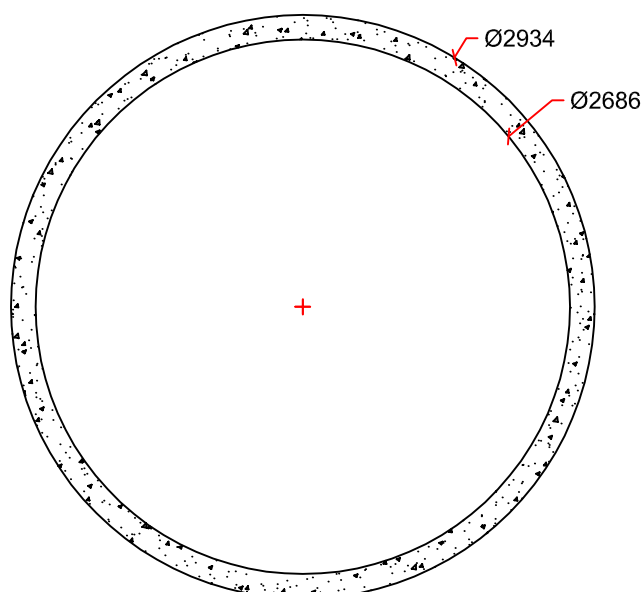
SECTION DETAIL
