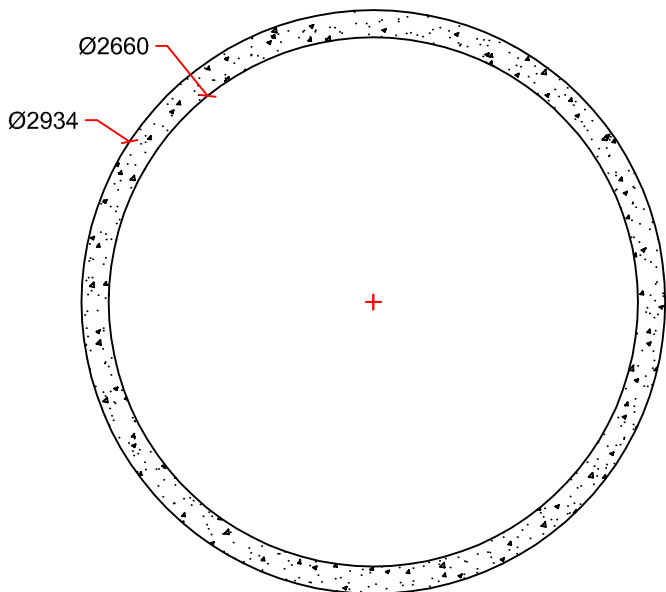
SECTION DETAIL
