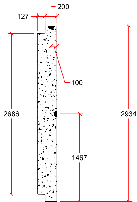
PROFILE VIEW
