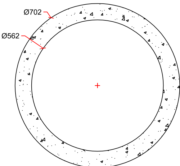
SECTION DETAIL
