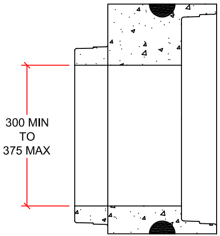
DECREASER
