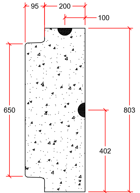
PROFILE VIEW
