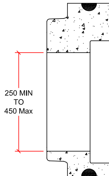
INCREASER
