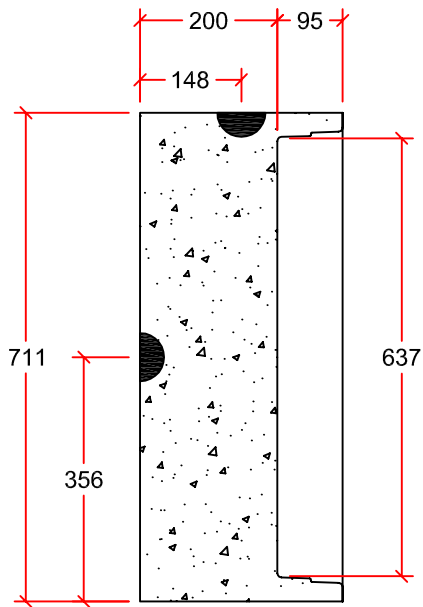
PROFILE VIEW
