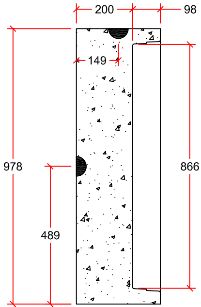
PROFILE VIEW
