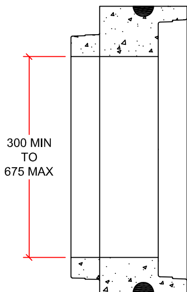
DECREASER
