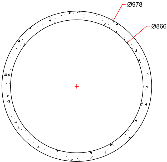
SECTION DETAIL
