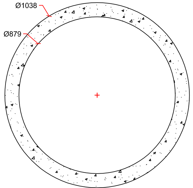
SECTION DETAIL
