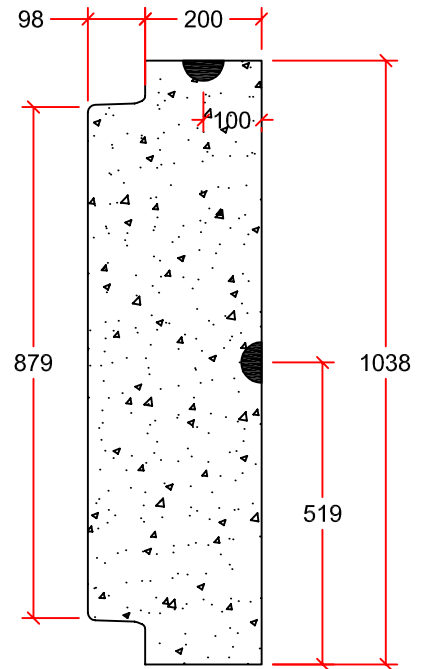
PROFILE VIEW
