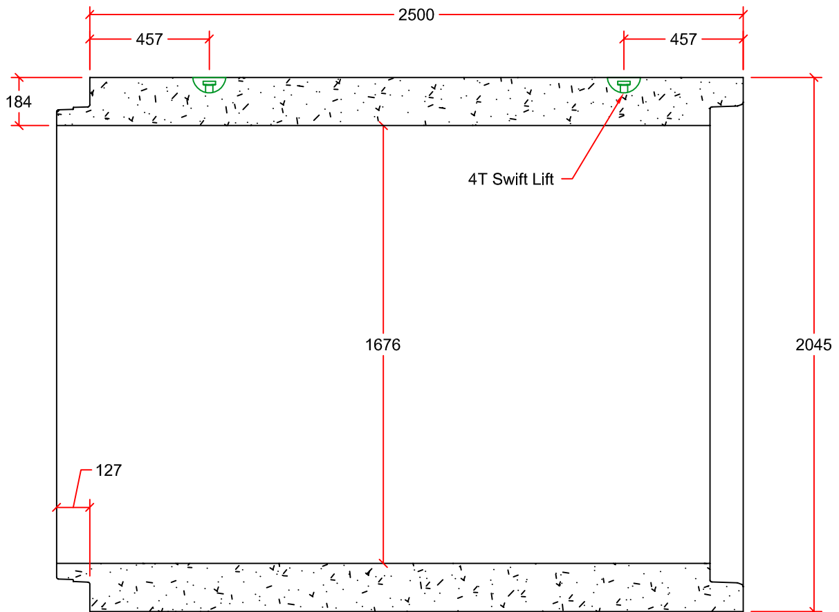
PIPE DETAIL
