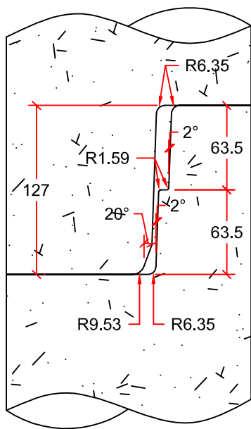
JOINT DETAIL
