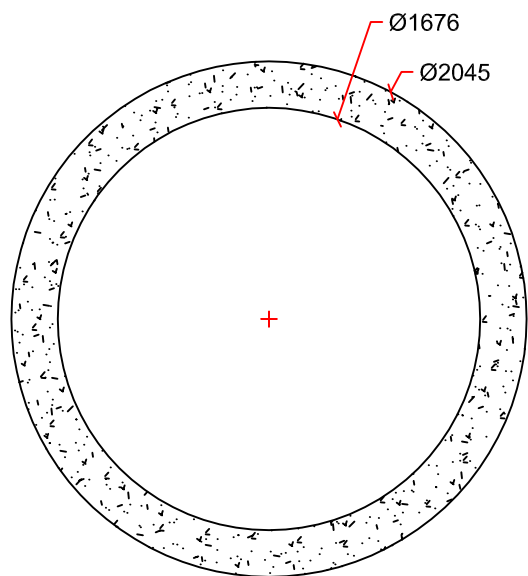
PIPE DETAIL
