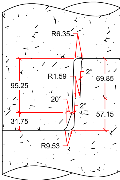
JOINT DETAIL
