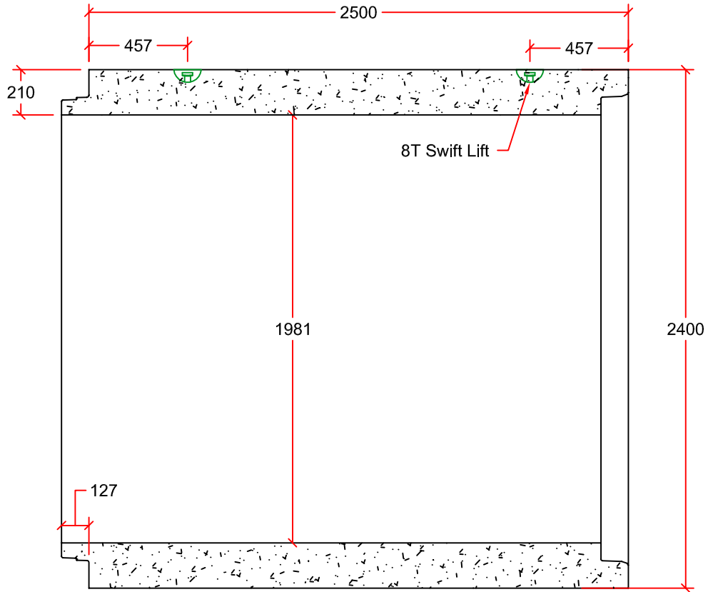
PIPE DETAIL
