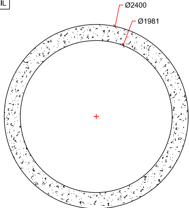
SECTION DETAIL
