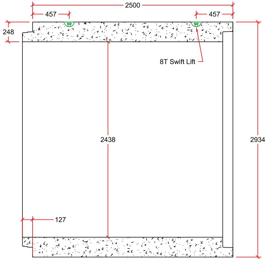
PIPE DETAIL
