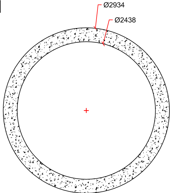
PIPE DETAIL
