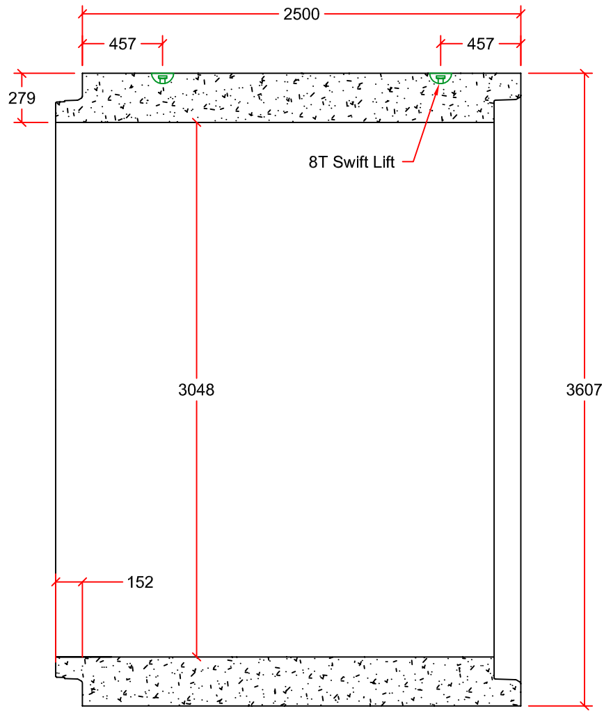
PIPE DETAIL
