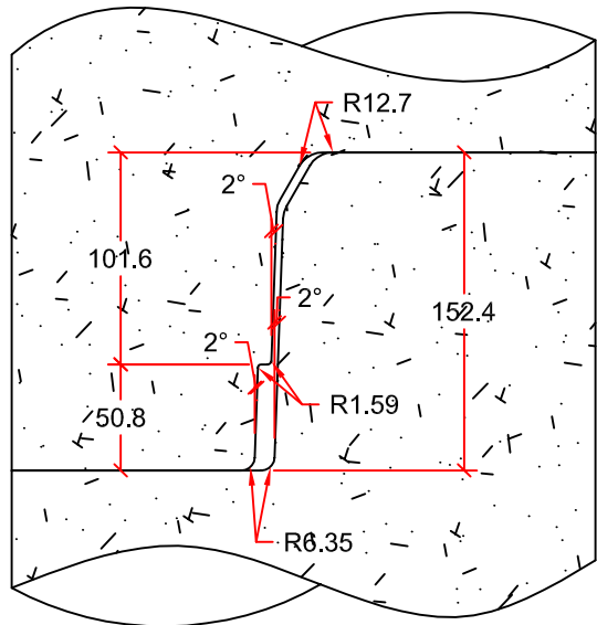
JOINT DETAIL
