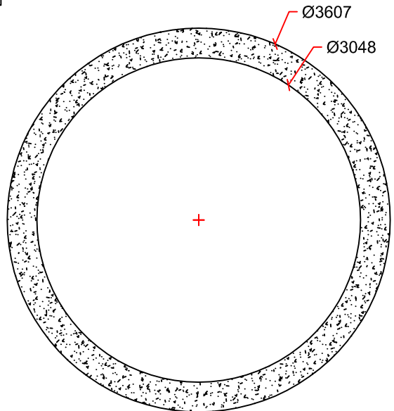
SECTION DETAIL
