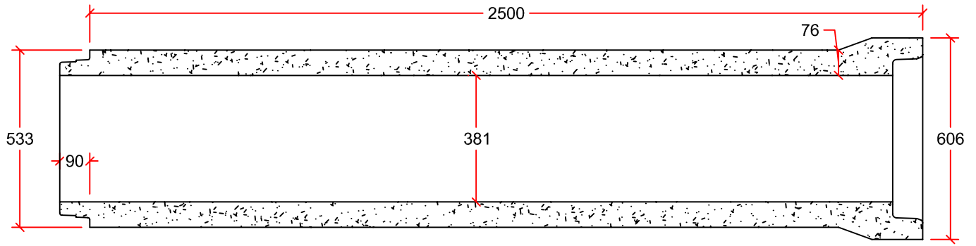
PIPE DETAIL
