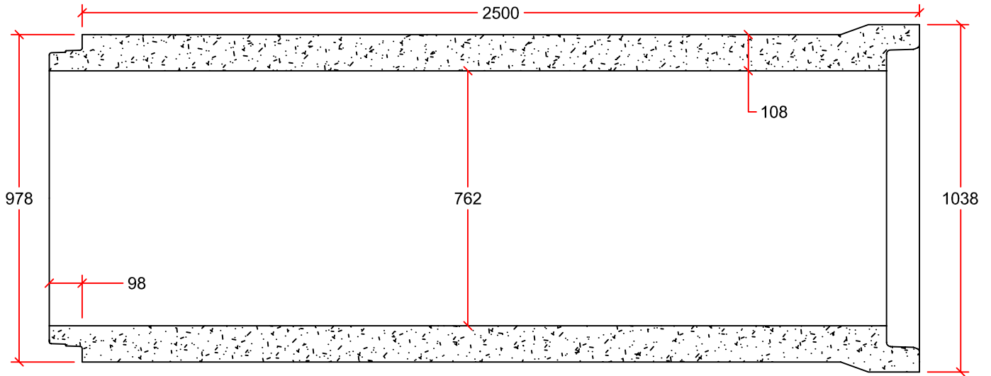
PIPE DETAIL
