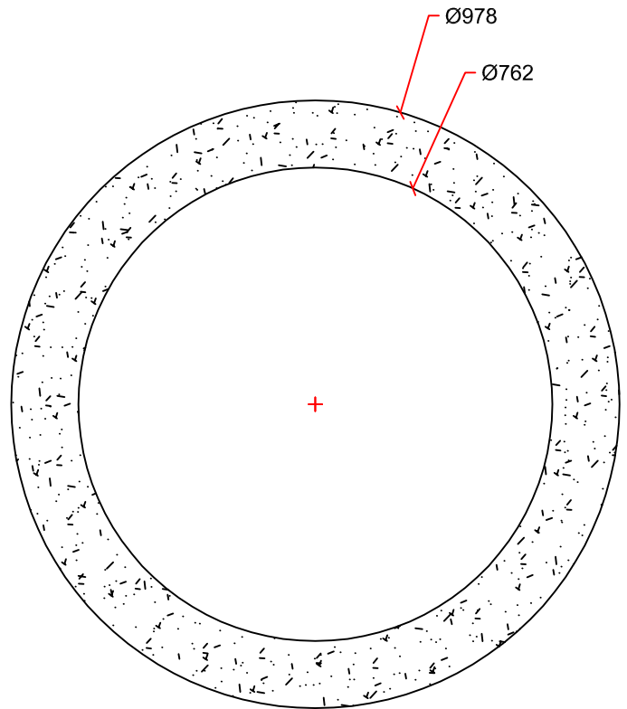
PIPE DETAIL
