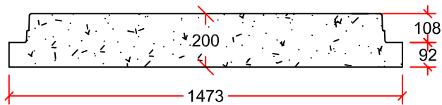
PROFILE VIEW
