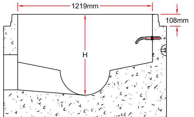
PROFILE VIEW
