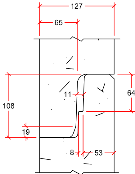
JOINT DETAIL
