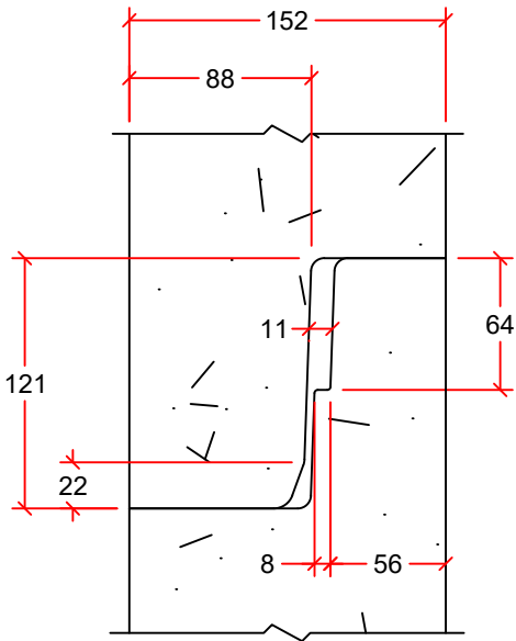
JOINT DETAIL
