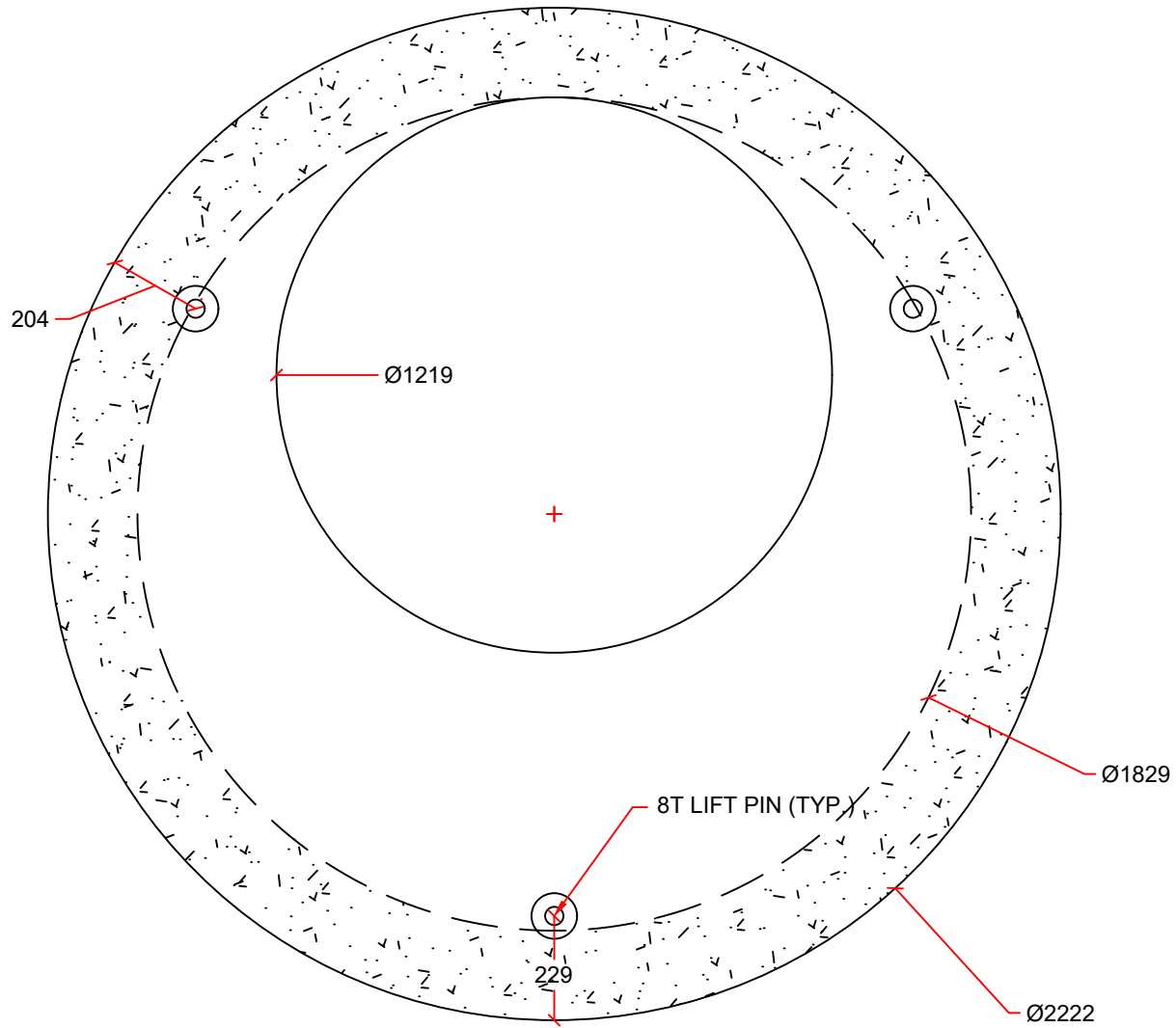
PLAN VIEW
