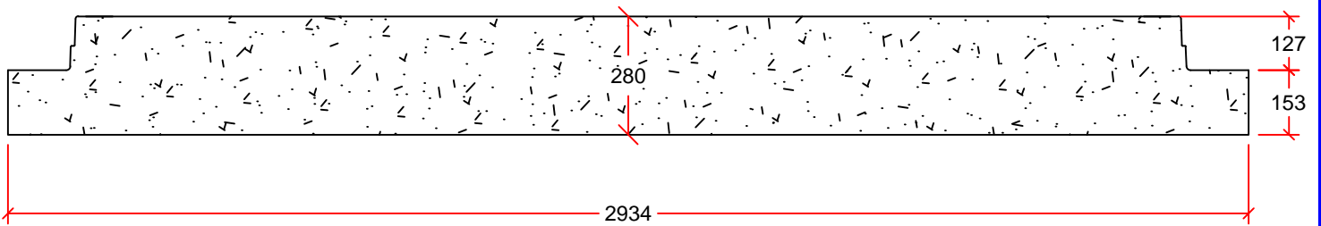
PROFILE VIEW
