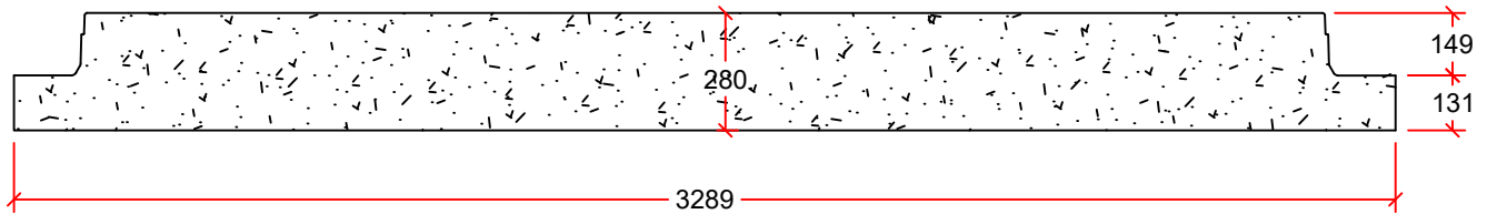
PROFILE VIEW
