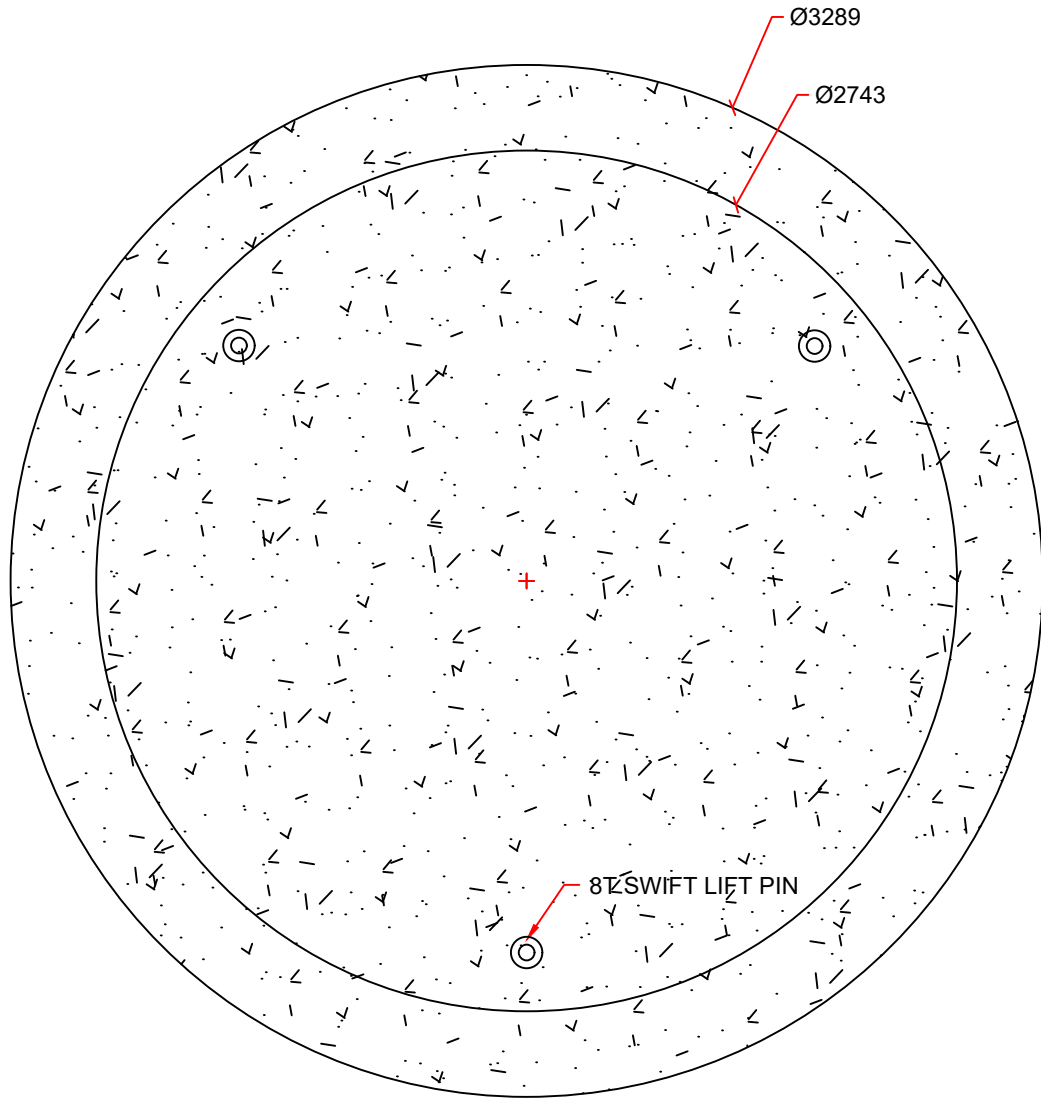
PLAN VIEW
