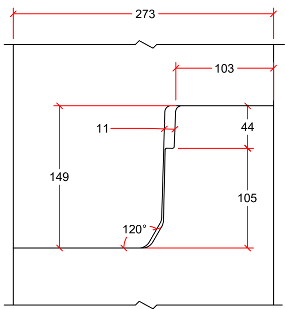
JOINT DETAIL
