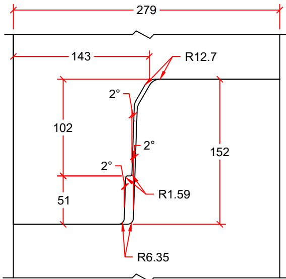
JOINT DETAIL
