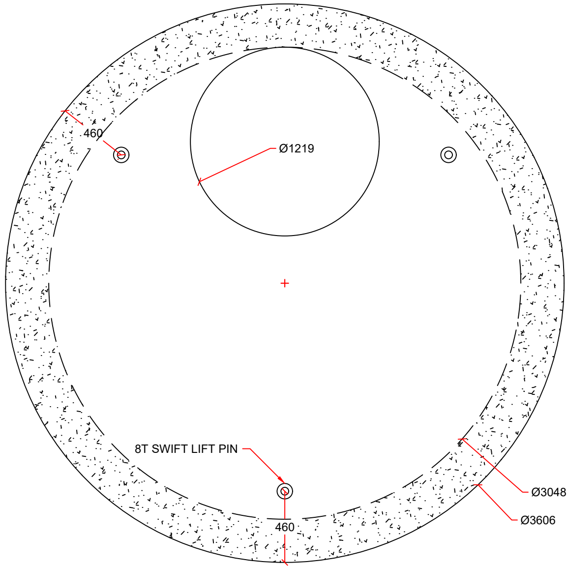
PLAN VIEW
