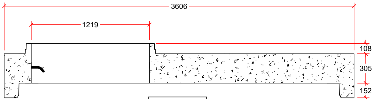
PROFILE VIEW
