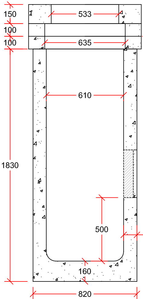
TYPICAL 600mm CATCH BASIN W/ 525 TOP
