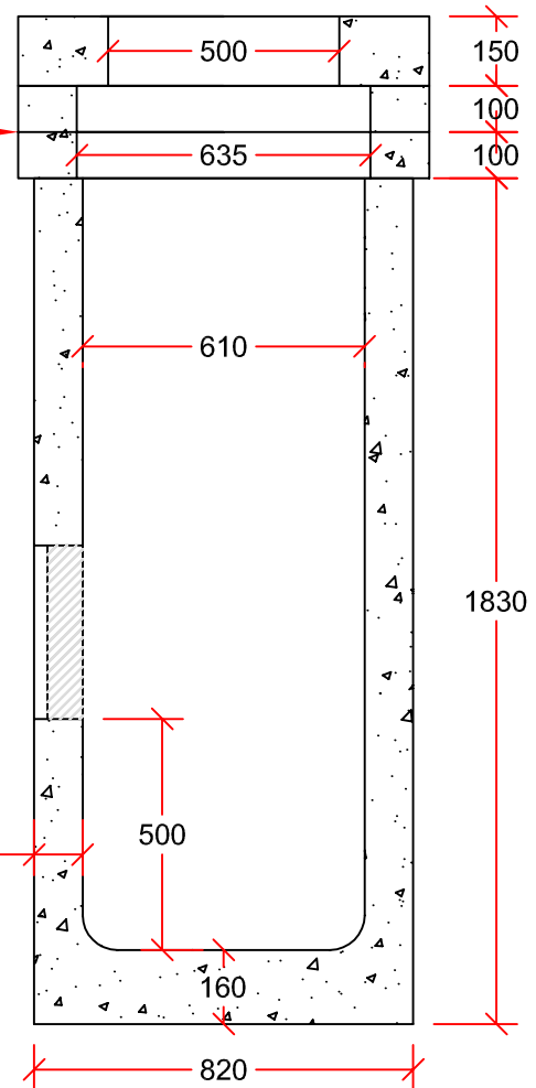
TYPICAL 600mm CATCH BASIN W/ K7 TOP
