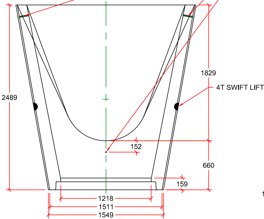
OUTLET SECTION
