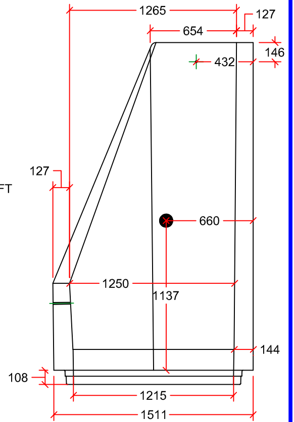
INLET SECTION
