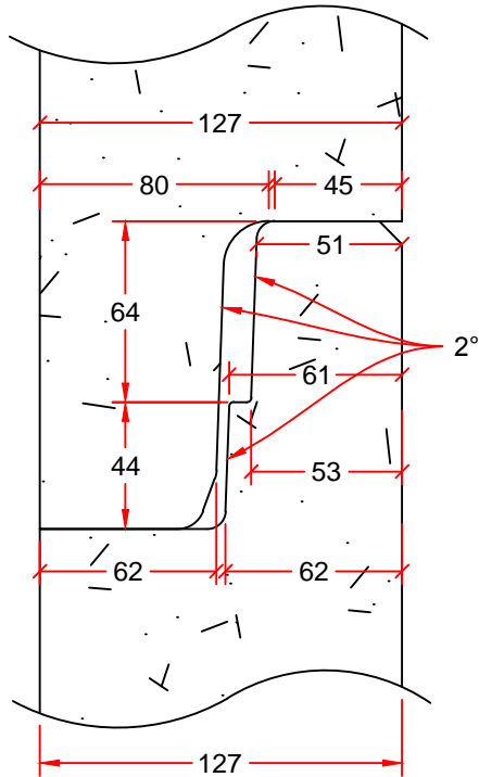
JOINT DETAIL
