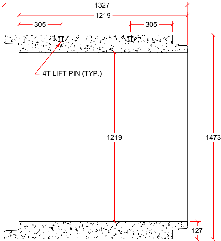
PIPE DETAIL
