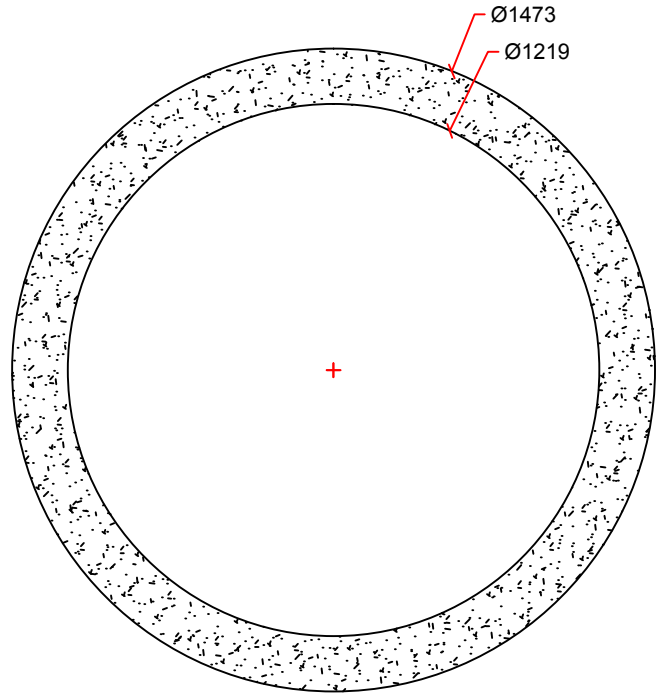
SECTION DETAIL
