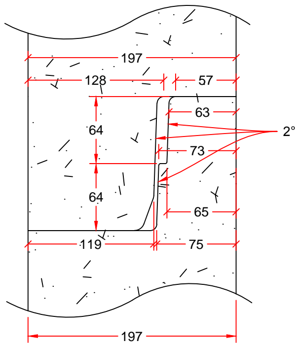
JOINT DETAIL
