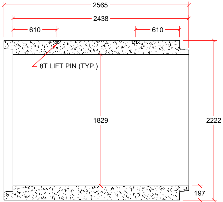
PIPE DETAIL
