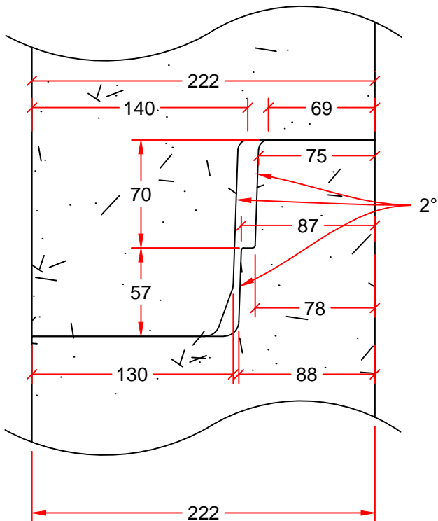
JOINT DETAIL
