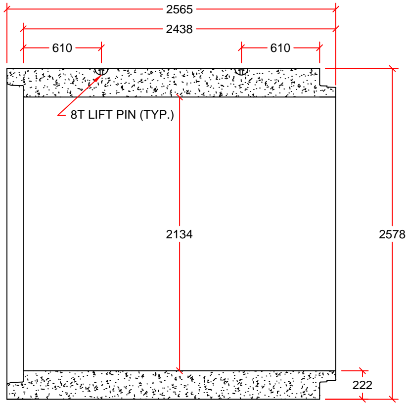
PIPE DETAIL
