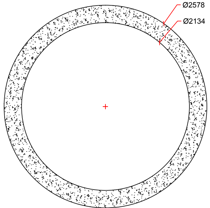
PIPE DETAIL
