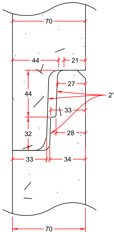
JOINT DETAIL
