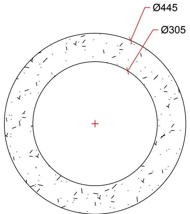
SECTION DETAIL
