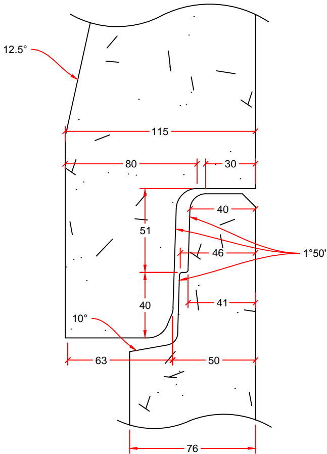
JOINT DETAIL
