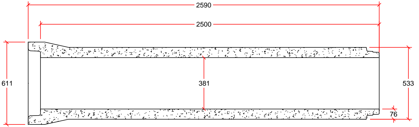
PIPE DETAIL
