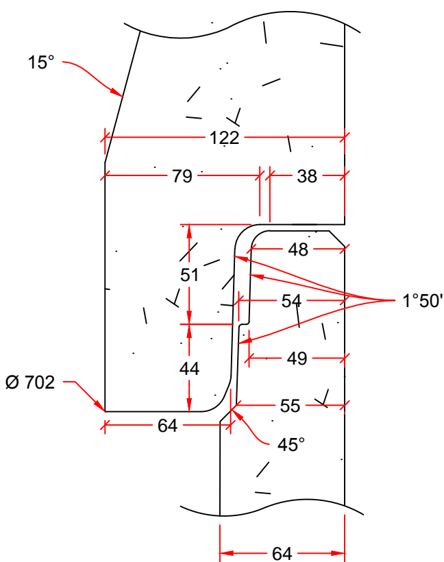
JOINT DETAIL
