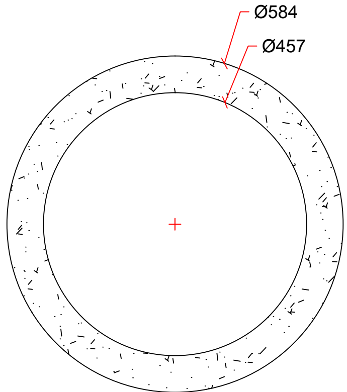
SECTION DETAIL
