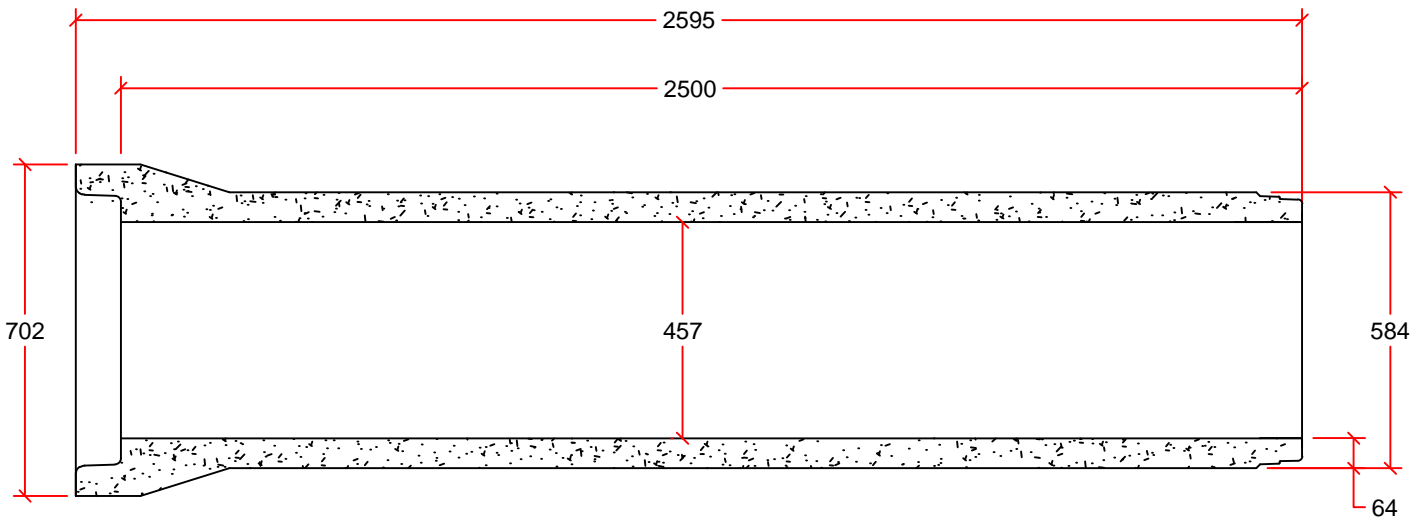
PIPE DETAIL
