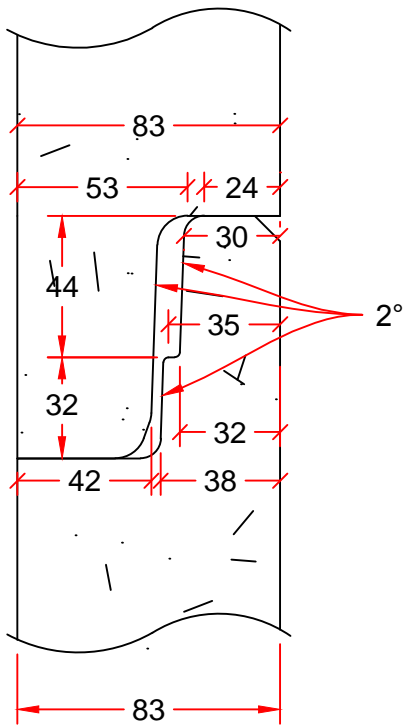
JOINT DETAIL
